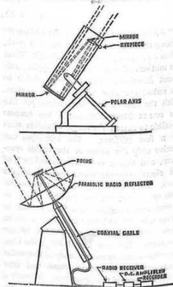
Fig. 2. An Optical and a Radio Telescope.
