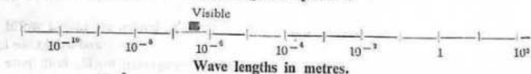
Fig. 1. Electromagnetic Spectrum.
